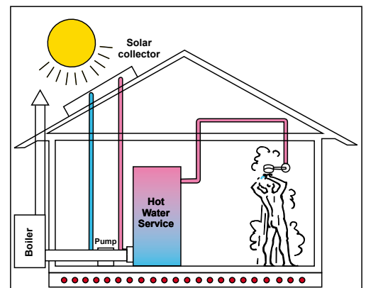
Infloor Slab Heating
